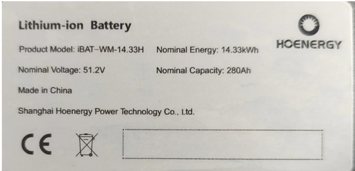
样品图片,铭牌(Sample photograph,label) -16
